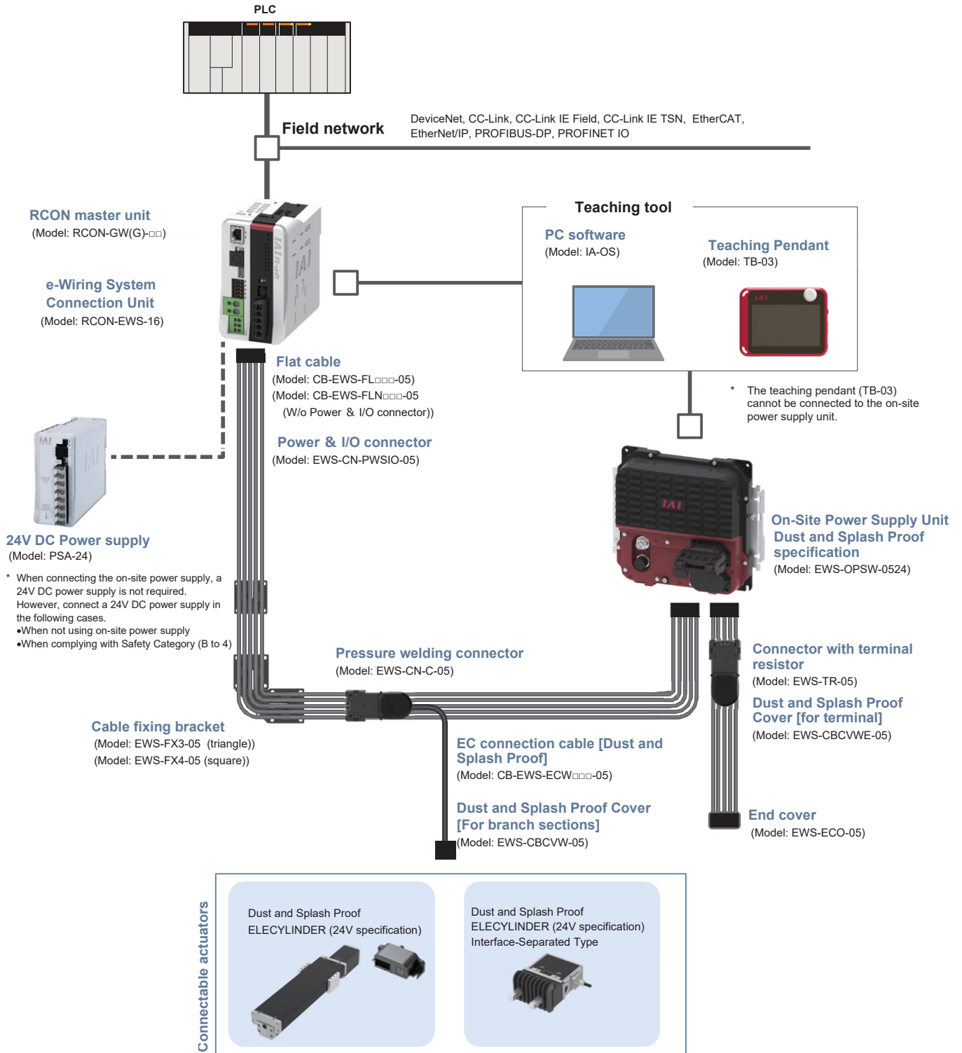
Fig. 4.1-2 Dust and Splash Proof Specification System Configuration
